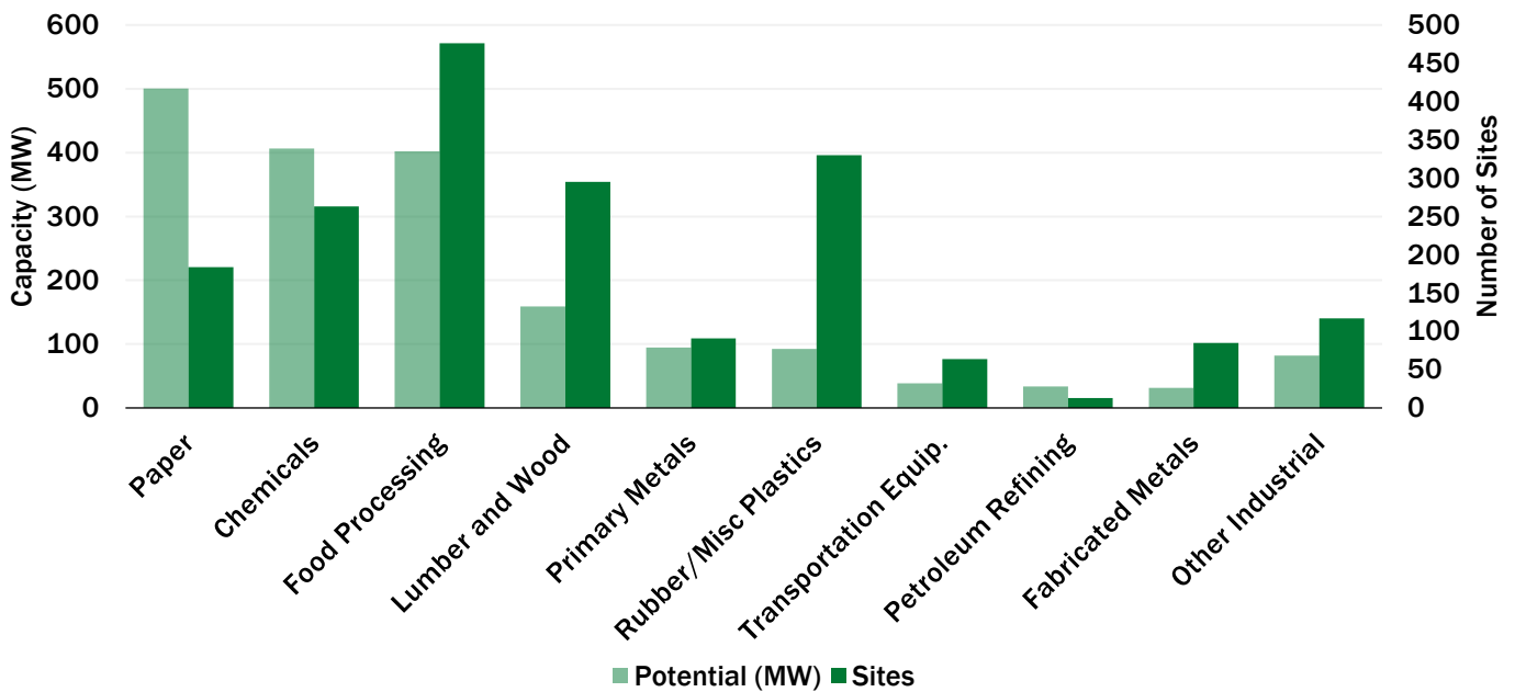
Wisconsin Technical Potential (MW) for Industrial CHP Applications
