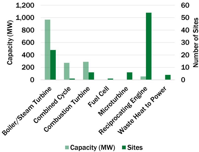
Wisconsin CHP by Technology
