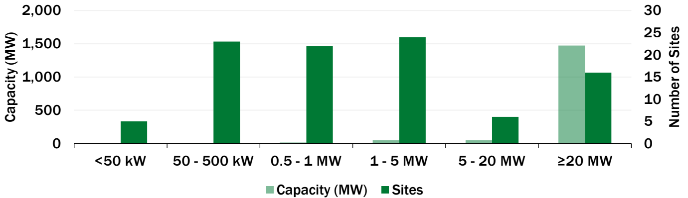
Wisconsin CHP by Size Range
