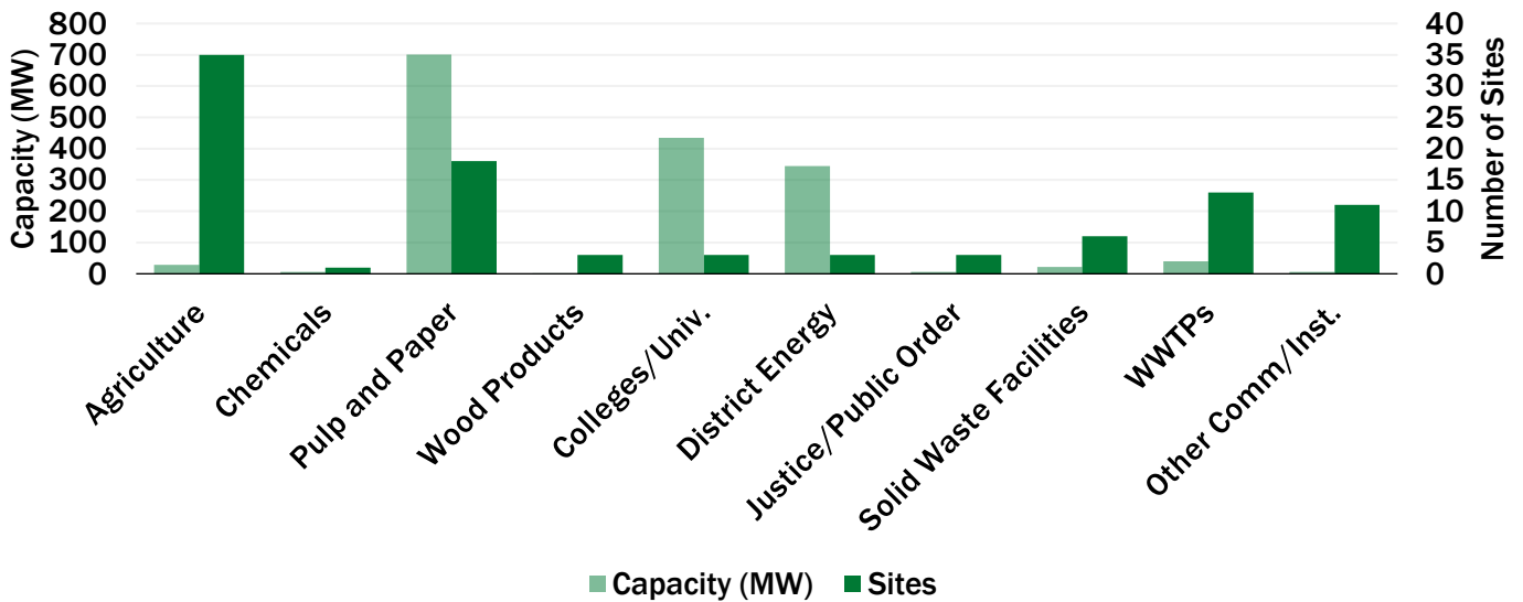
Wisconsin CHP by Application
