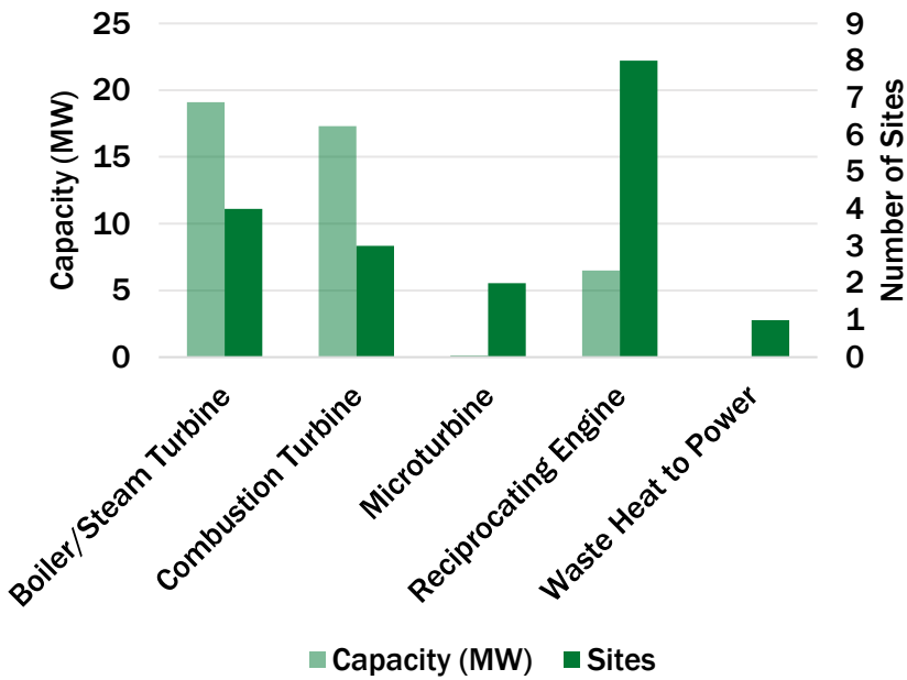
New Hampshire CHP by Technology
