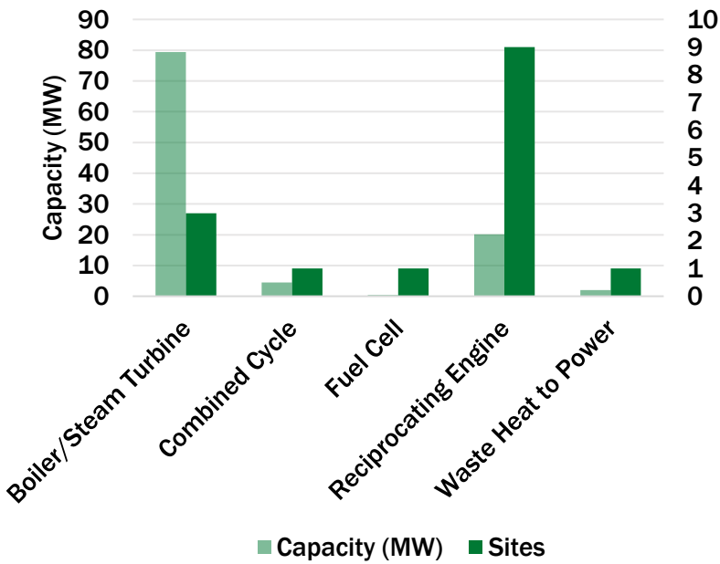
Nebraska CHP by Technology
