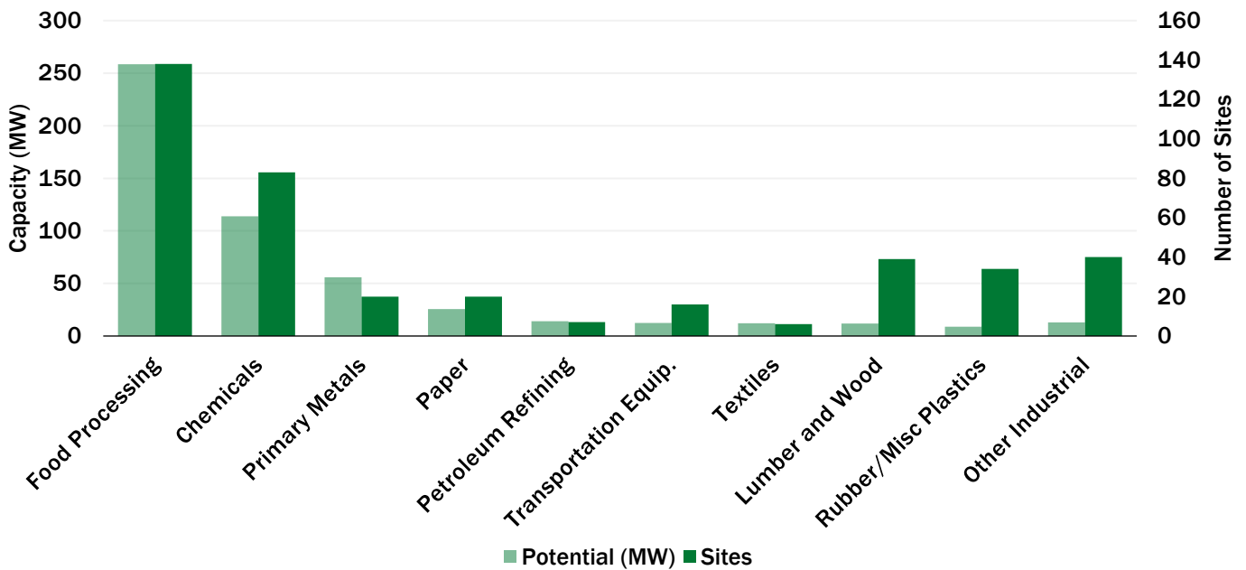
Nebraska Technical Potential (MW) for Industrial CHP Applications
