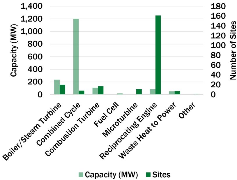
Massachusetts CHP by Technology
