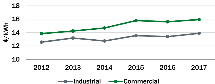
Massachusetts Average Electricity Prices
