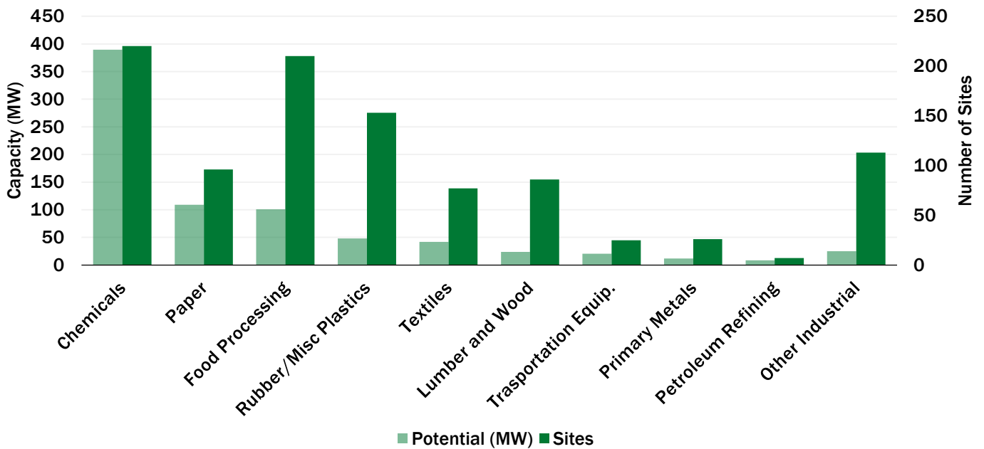
Massachusetts Technical Potential (MW) for Industrial CHP Applications
