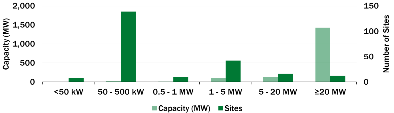
Massachusetts CHP by Size Range
