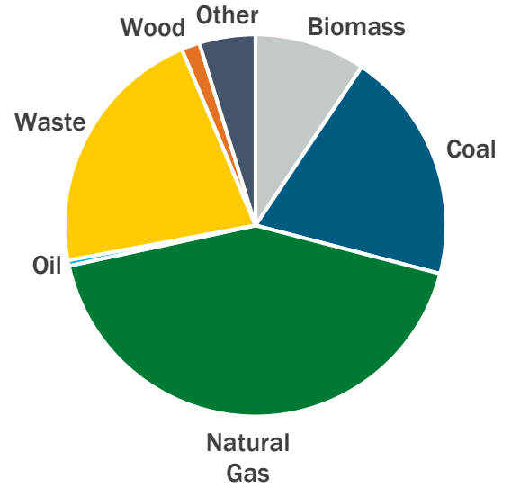
Florida CHP Capacity (MW) by Fuel
