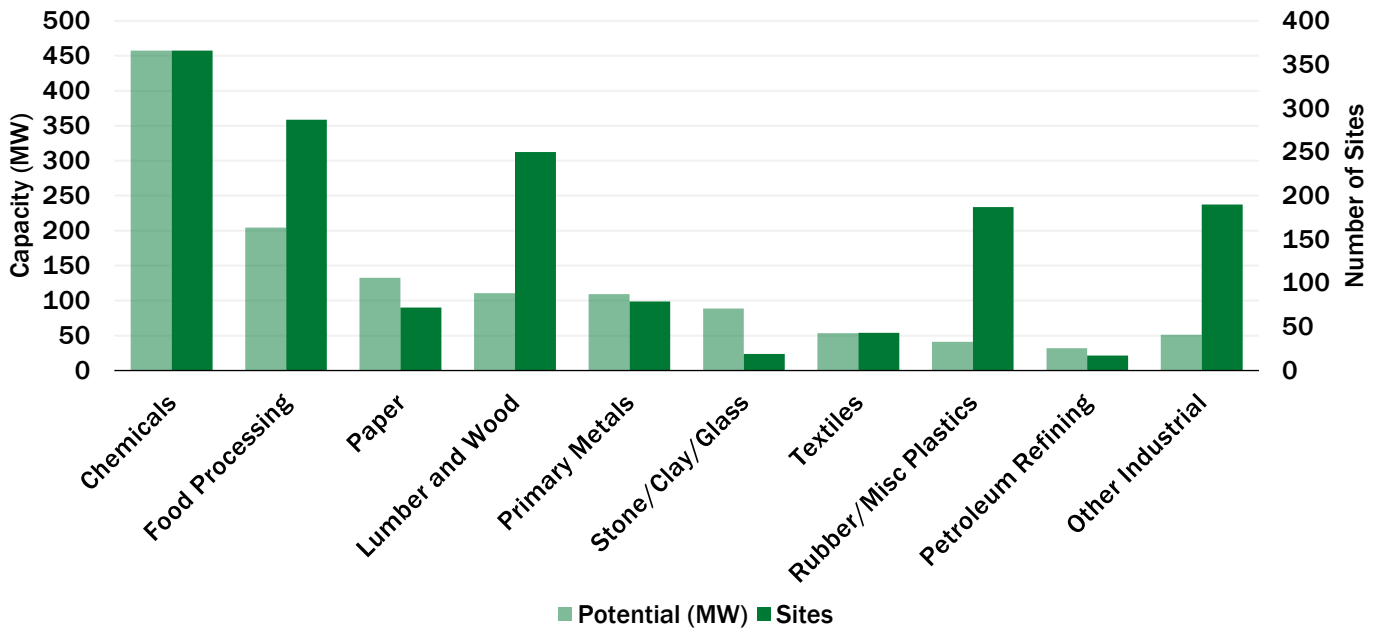
Florida Technical Potential (MW) for Industrial CHP Applications
