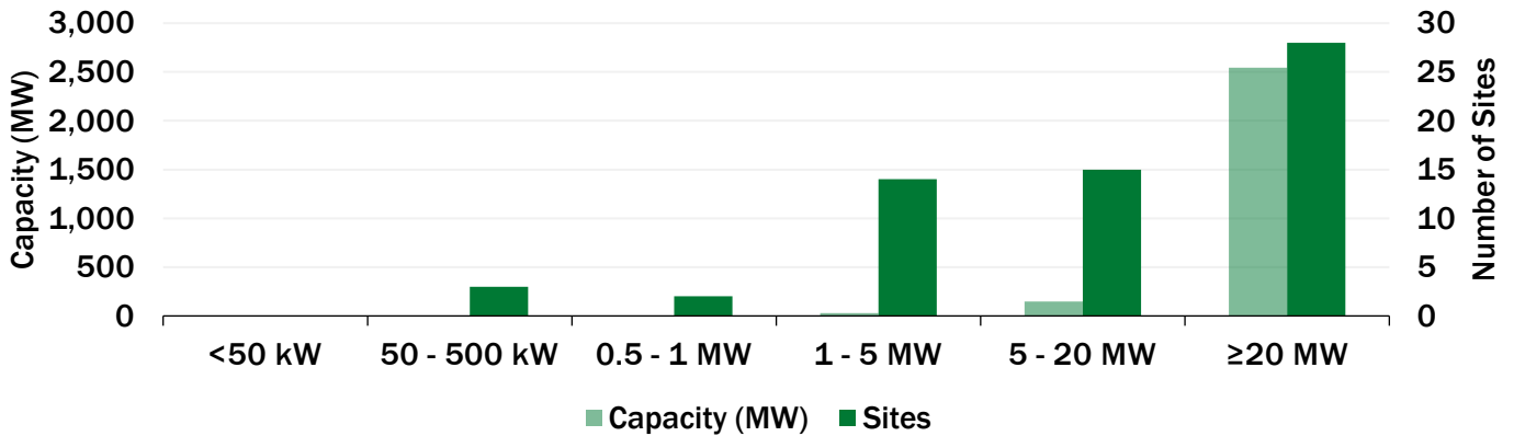
Florida CHP by Size Range
