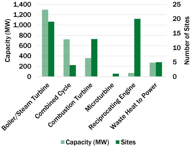
Florida CHP by Technology
