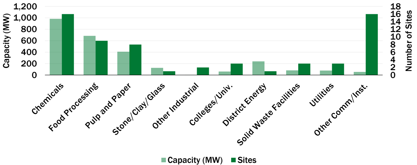
Florida CHP by Application
