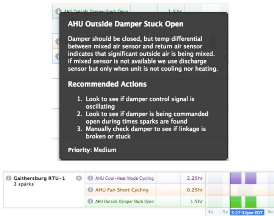
FIGURE 5: EXAMPLE SCREENSHOT (SKYFOUNDRY) OF A FDD TOOL, SHOWING FAULTS AND RECOMMENDED ACTIONS
