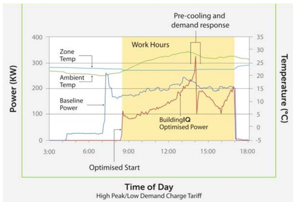
FIGURE 6: EXAMPLE (BUILDING IQ) OF HOW AN ASO TOOL WORKS ON AN HVAC SYSTEM IN A TYPICAL BUILDING DURING A TYPICAL DAY
