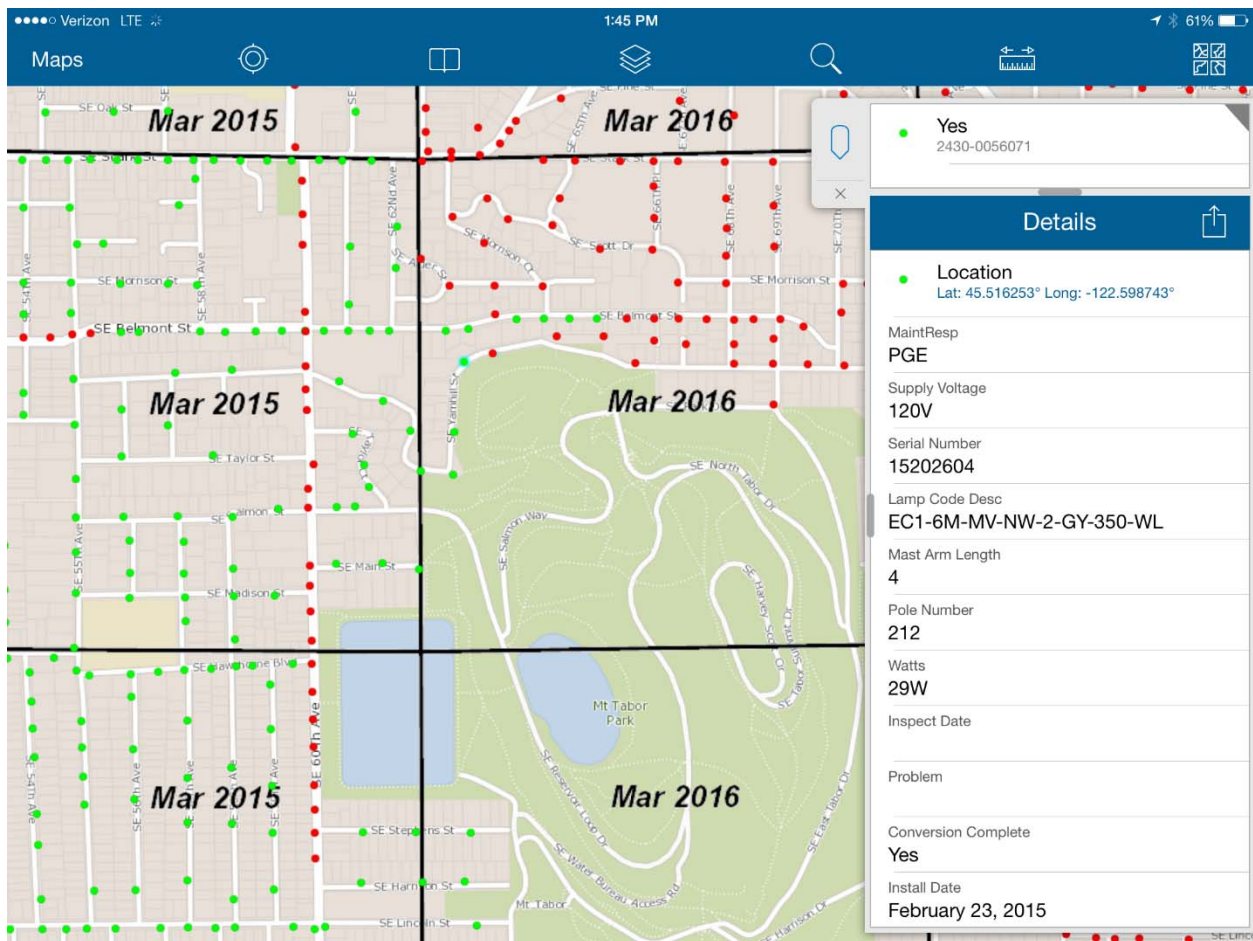
Figure 1 -Editable details for cobrahead luminaire. The contractor adds serial number and install date, as well as any comments as necessary. The contractor is also able to check pole number in GIS against pole number on pole tag.
